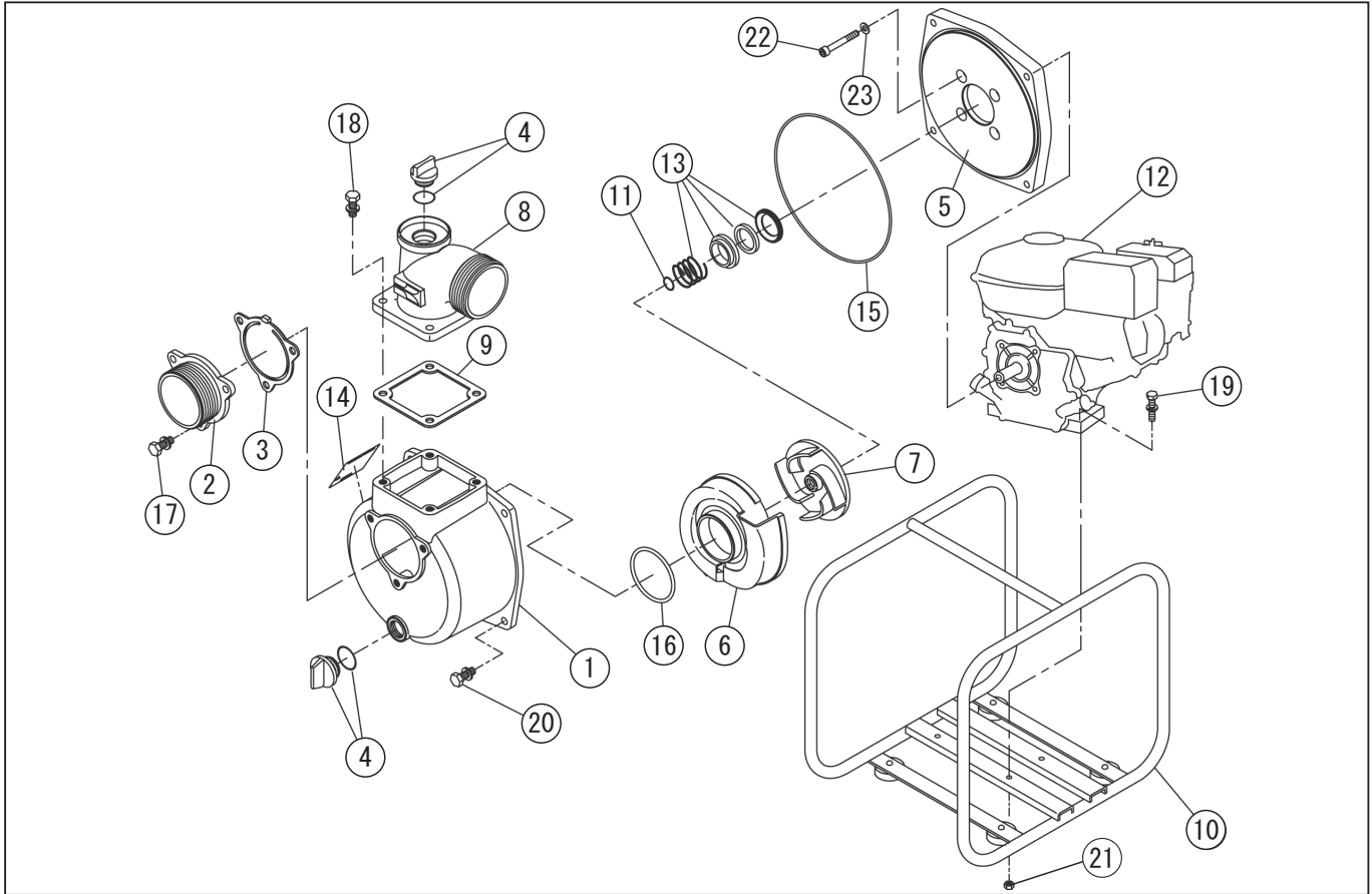
DWG No.066864301 MODEL : SEH-50X FORM : SEH-50X-BAJ-6(GX120UT2)
