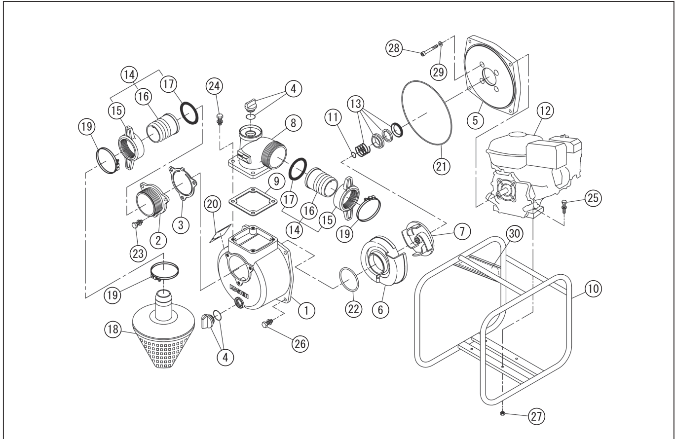
DWG No.012933801 MODEL : SEH-50X FORM : SEH-50X-BGD-0 (GX120T2)
