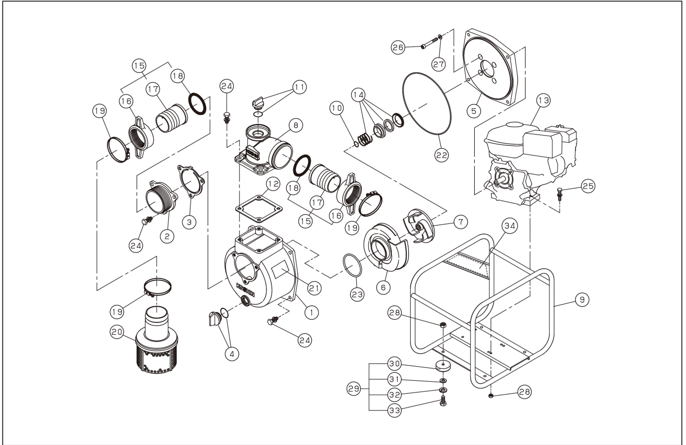
DWG No.012904915 MODEL : SEH-80X FORM : SEH-80X-BER-4(GX160T2)
