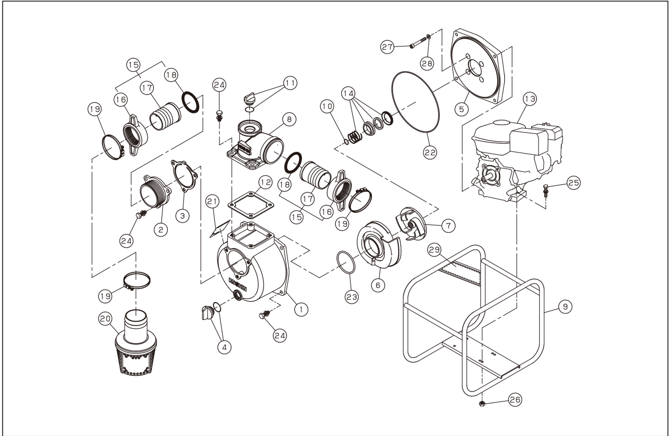
DWG No.012923611 MODEL : SEH-80X FORM : SEH-80X-BFG-2(GX160T2)
