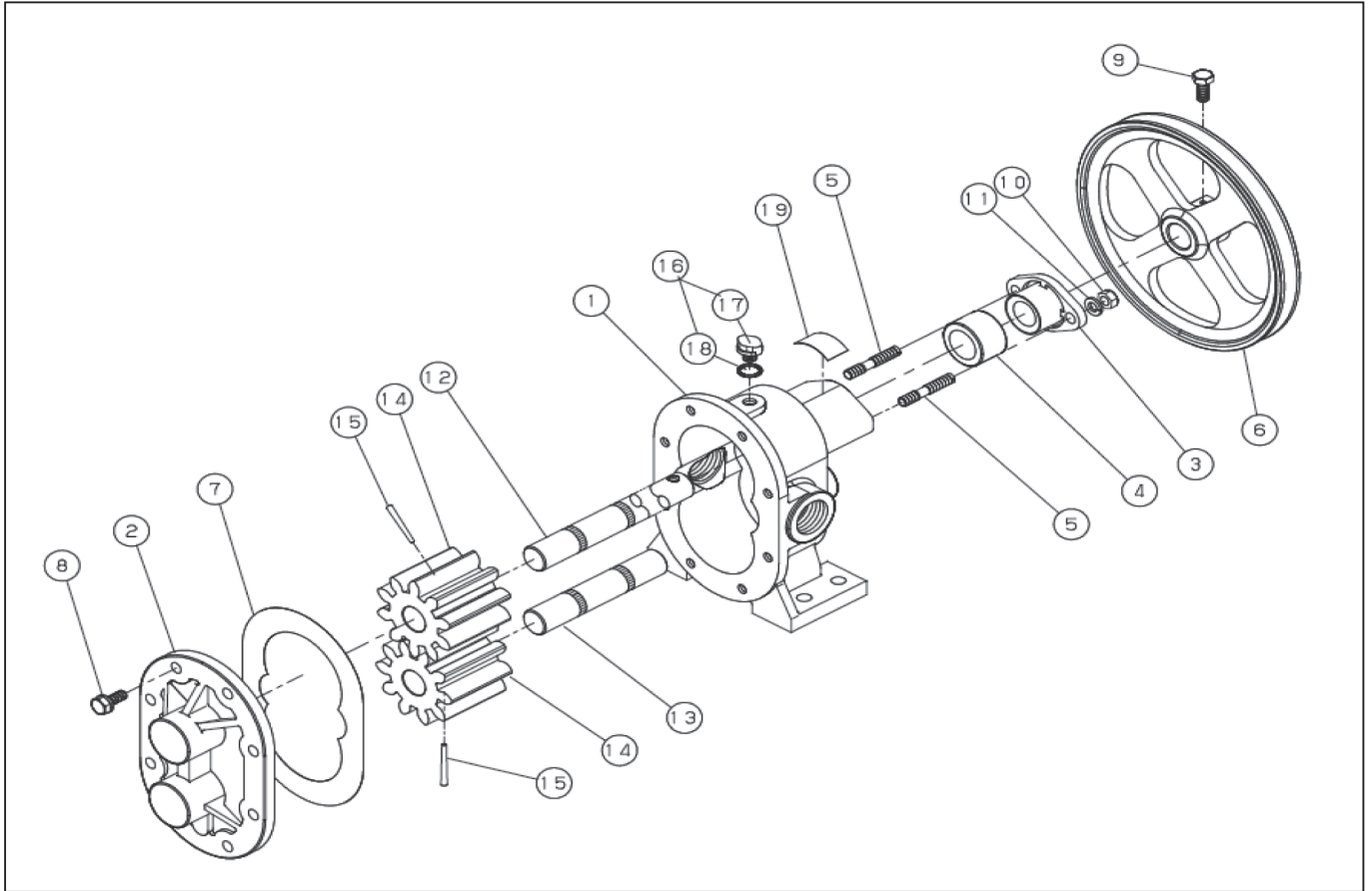
DWG No.002857511 MODEL:GB-20 FORM:GB-20-BAA-1
