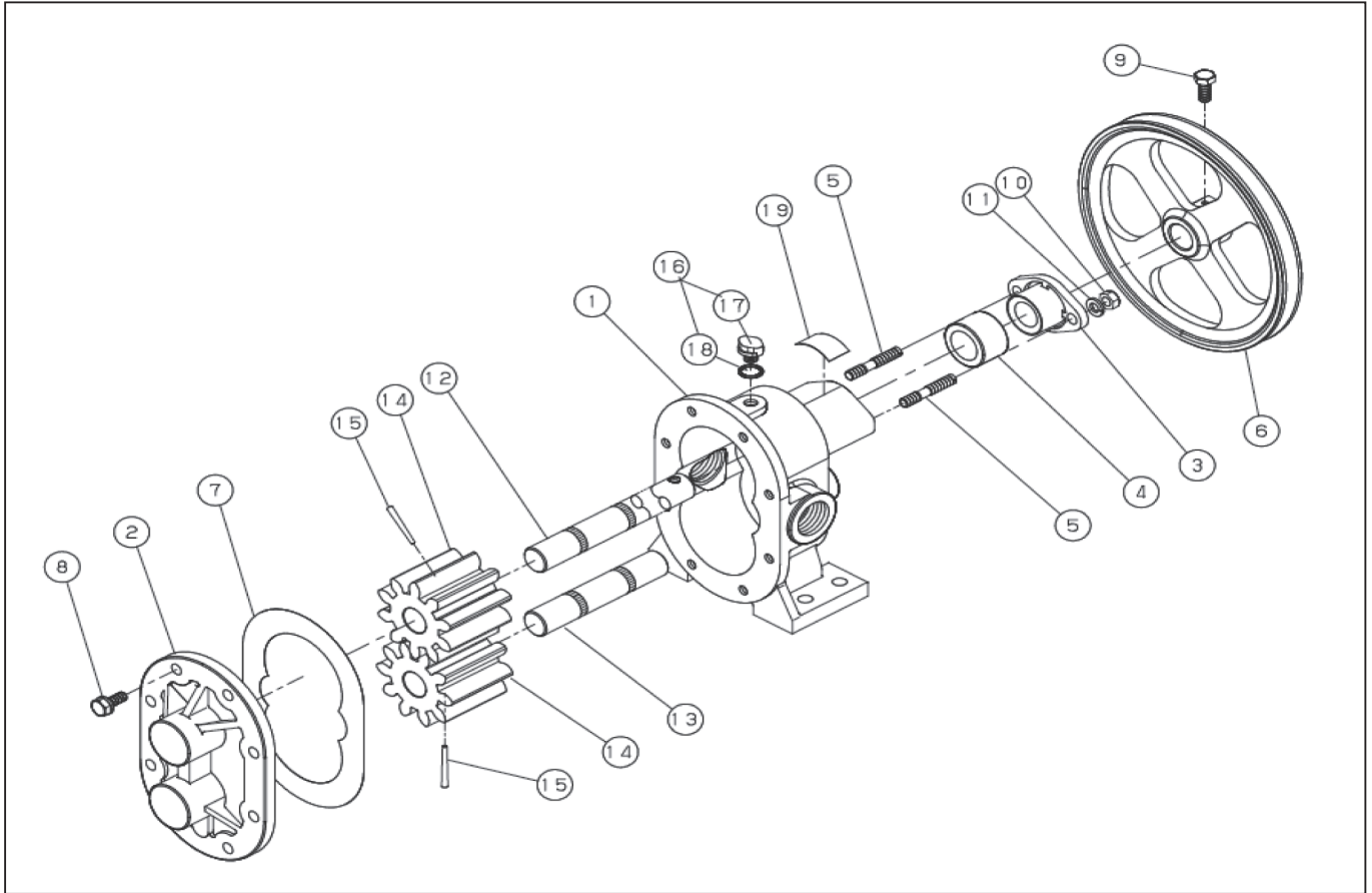
DWG No.002852010 MODEL:GB-25 FORM:GB-25-BAA-1
