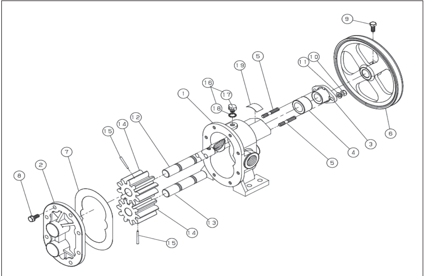
DWG No.002857708 MODEL:GC-13 FORM:GC-13-BAA-1
