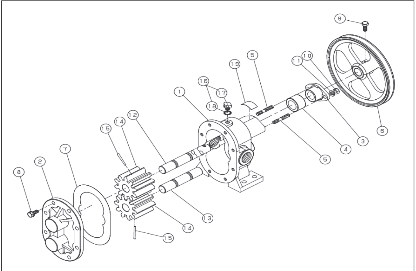
DWG No.002857708 MODEL:GC-20 FORM:GC-20-BAA-1
