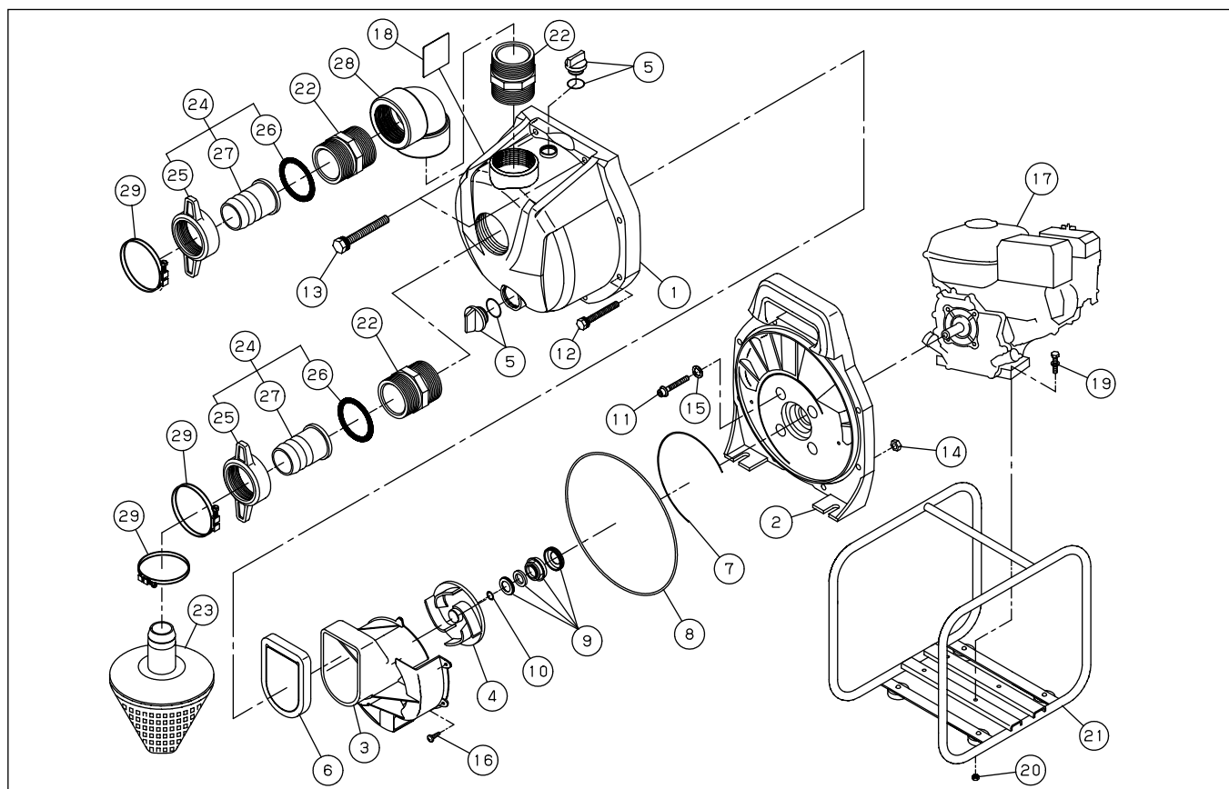
PGM-50G-AAA-0 (0138515) 部品表
