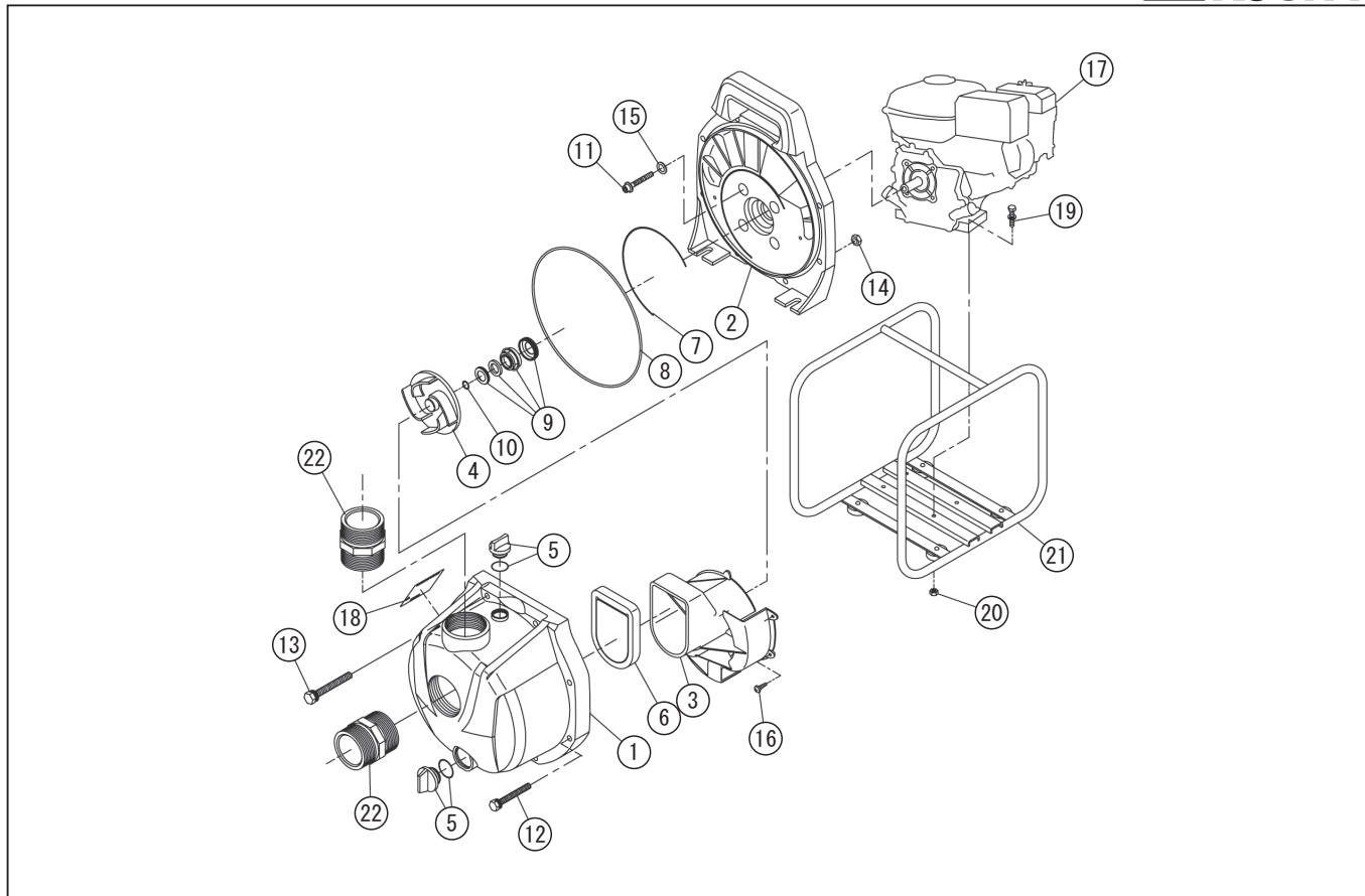
DWG No.013851404 MODELE : PGM-50G FORM : PGM-50G-BAA-2 (GT400)
