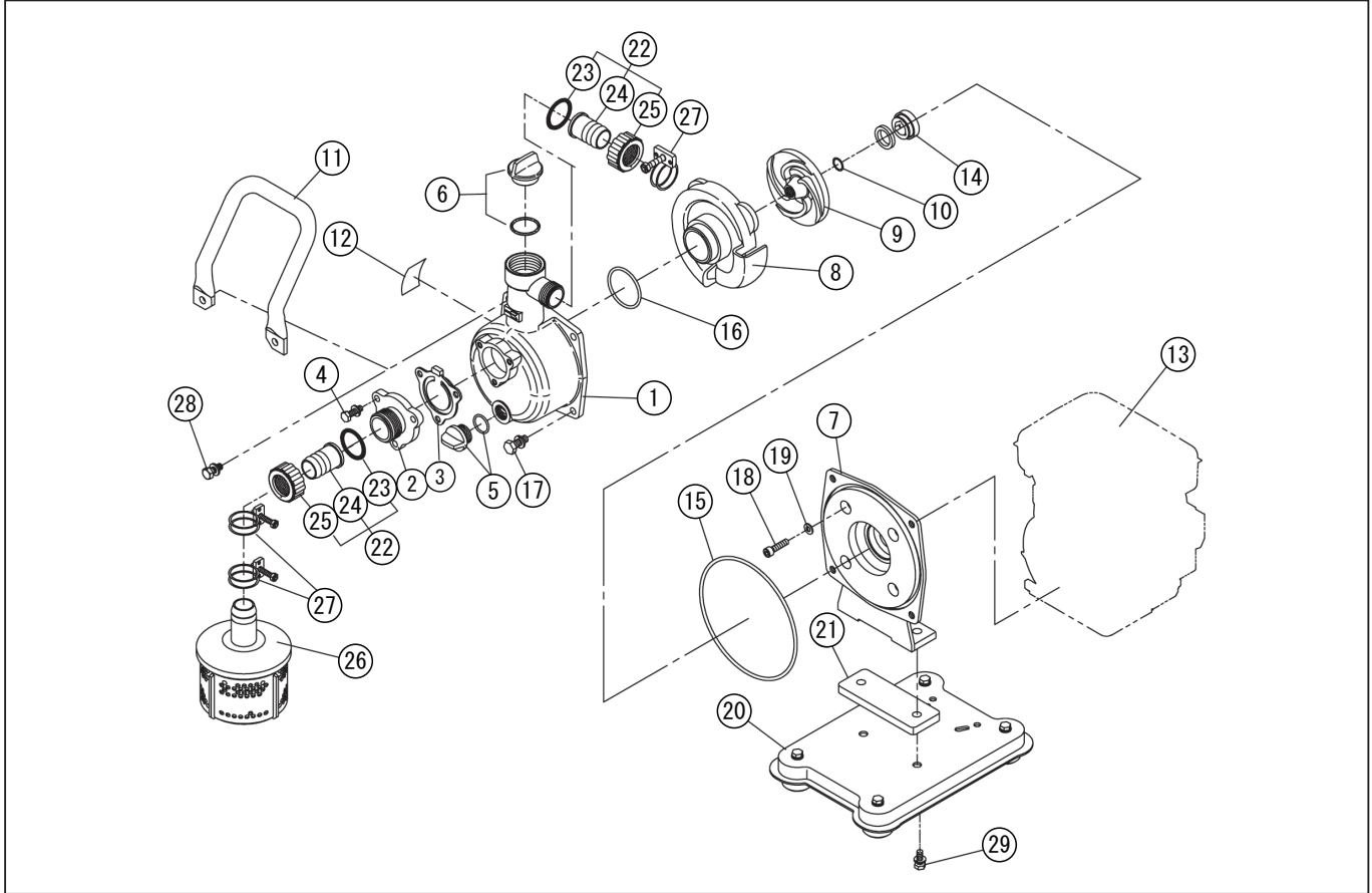
DWG No.012887505 MODEL : SE-25FH FORM : SE-25FH-BAA-1
