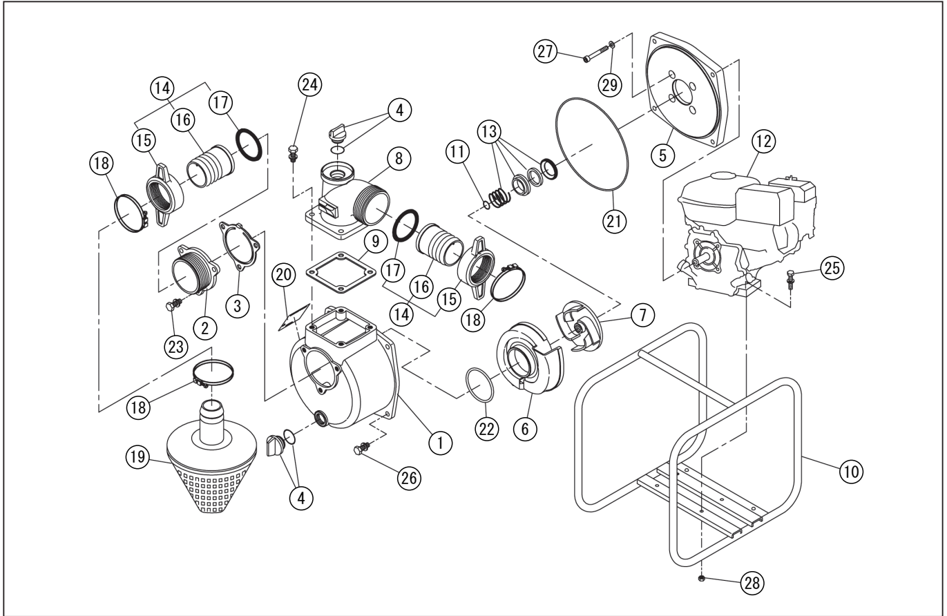
DWG No.011929718 MODEL : SE-50XK FORM : SE-50X-BAF-2 (EY15-3)
