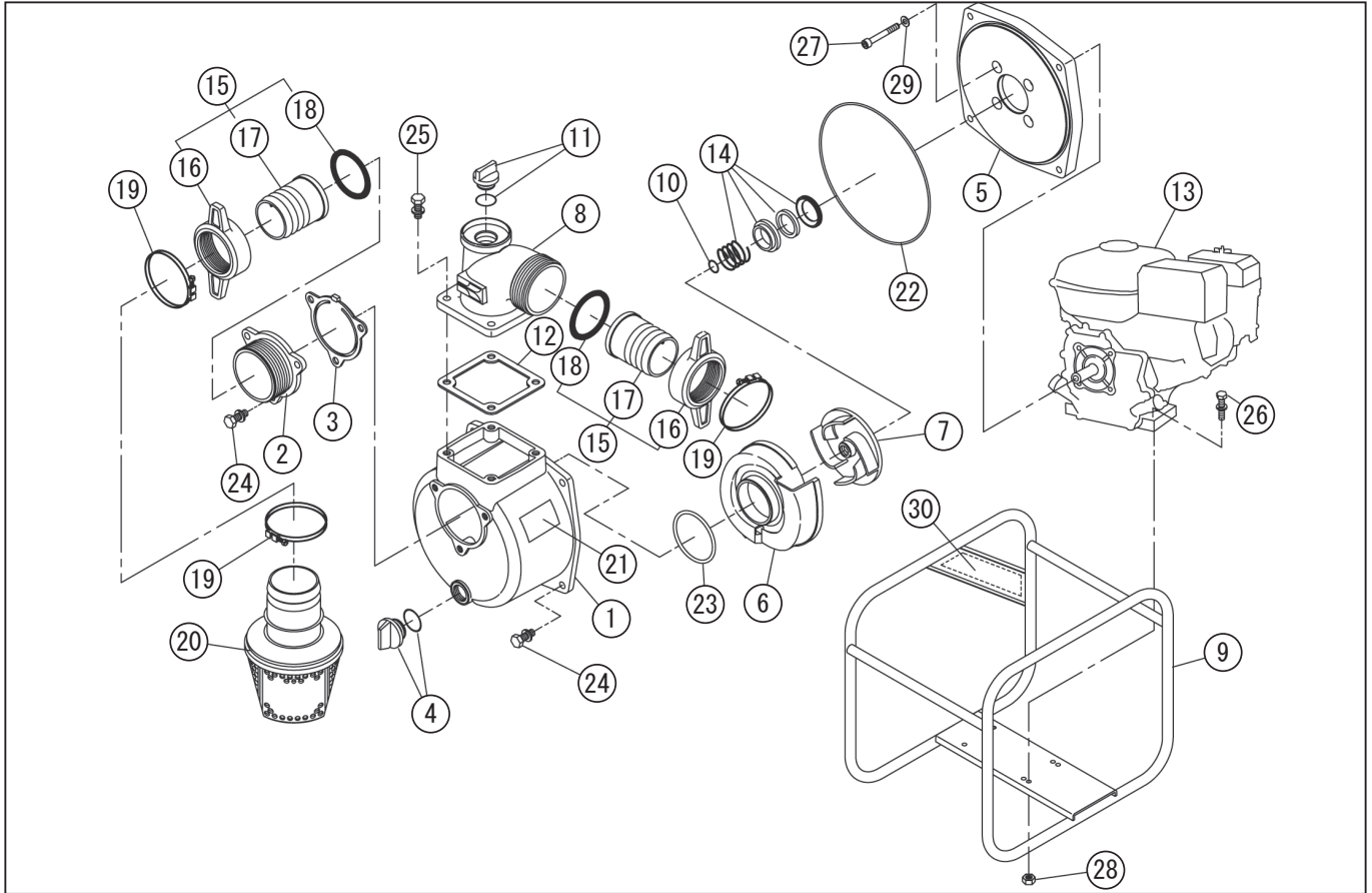
DWG No.012871813 MODEL:SE-80X FORM:SE-80X-BCN-3 (EY20-3)
