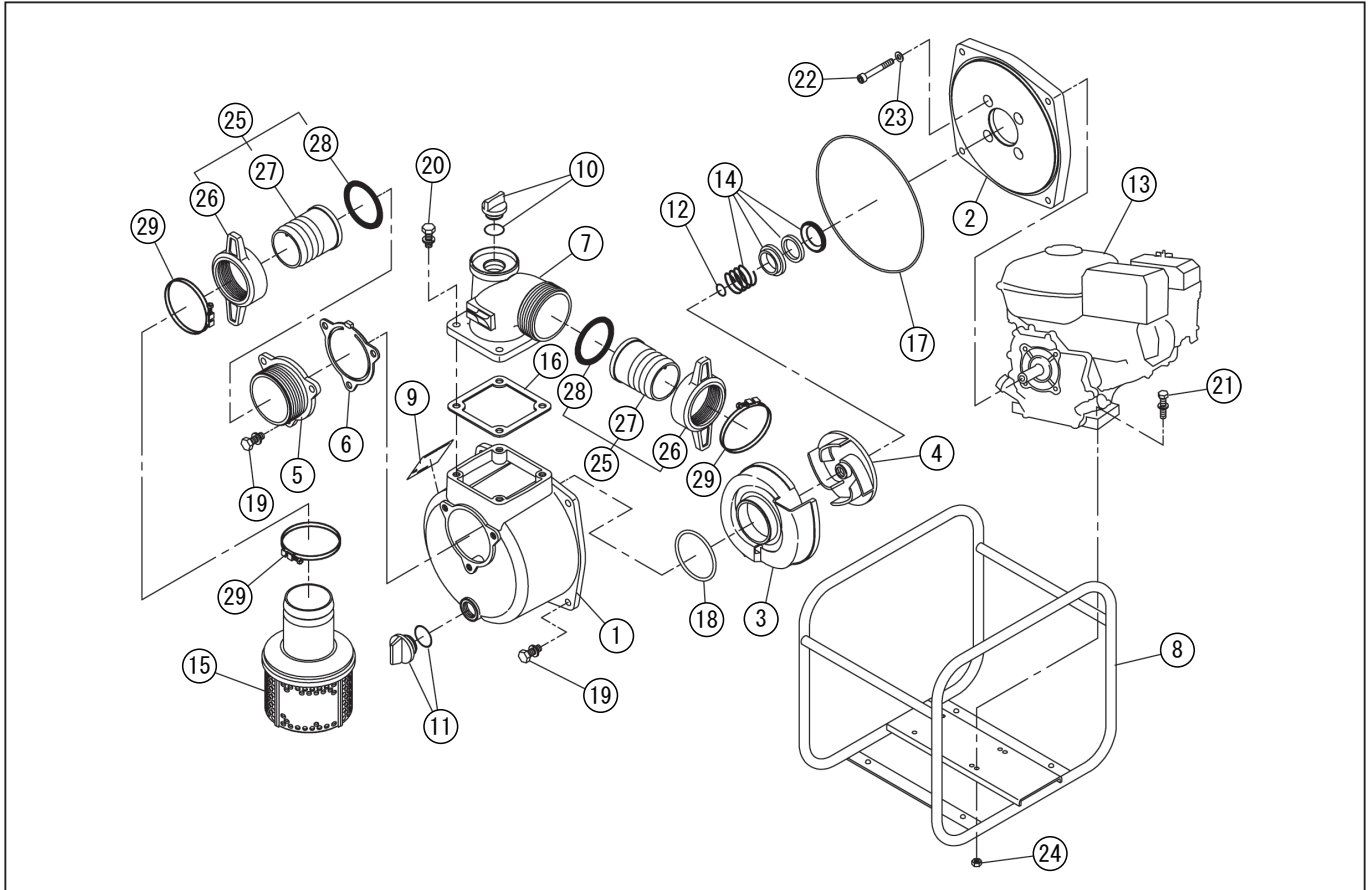
DWG No.066862203 MODEL : SE-80XK FORM : SE-80X-BED-0 (EY20-3)
