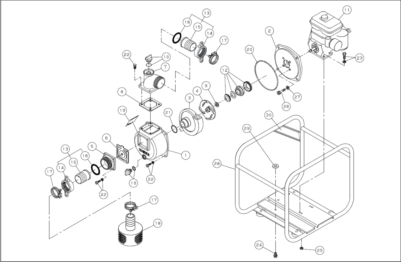
DWG No.012867615 MODEL : SEH-100X FORM : SEH-100X-BAE-4 (GX240UT2)
