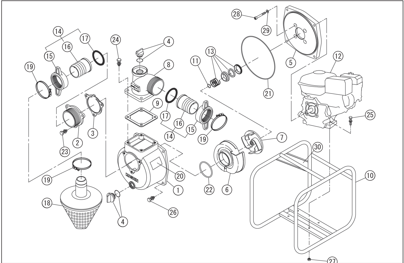
DWG No.012924103 MODEL : SEH-50X FORM : SEH-50X-BFZ-1
