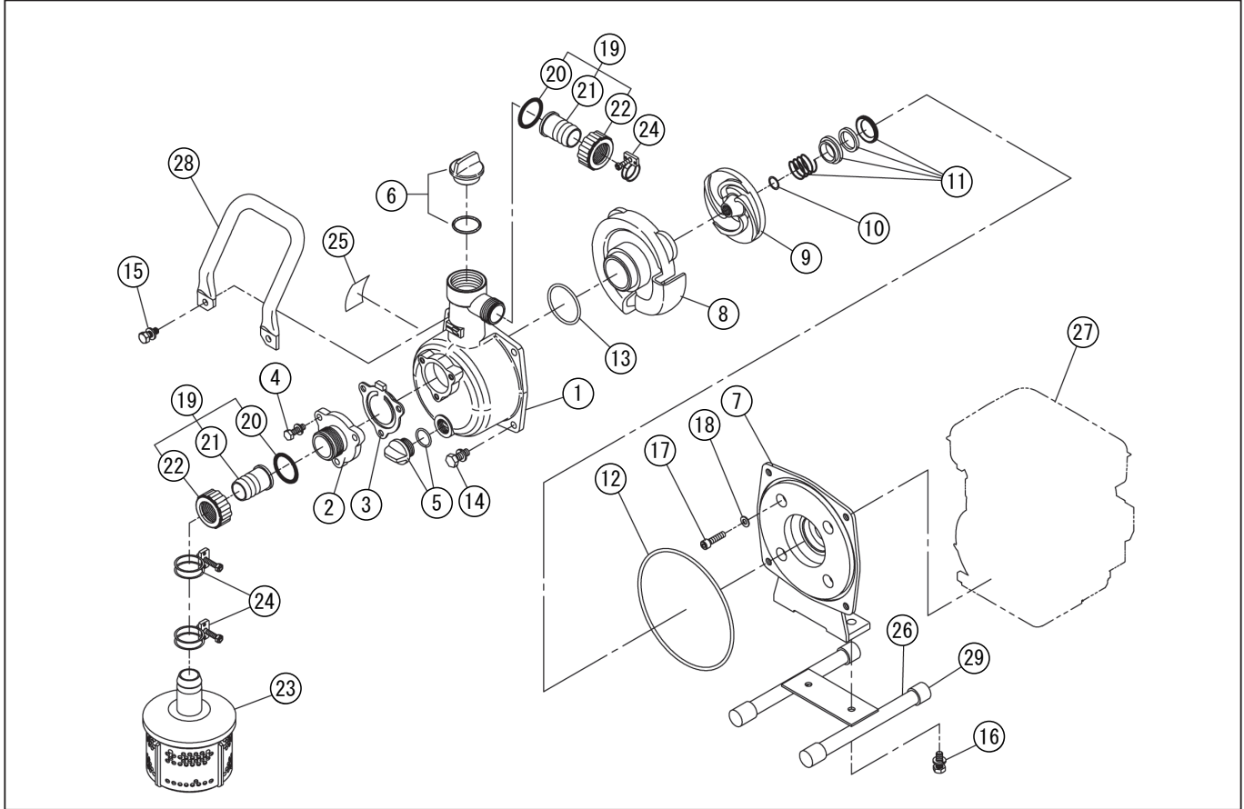
DWG No.012901702 MODELE:SEM-25E FORM:SEM-25E-BAF-0
