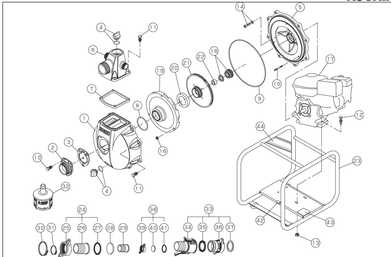
DWG No.013852702 MODEL:SERV-50Z FORM:SERV-50Z-BAA-0
