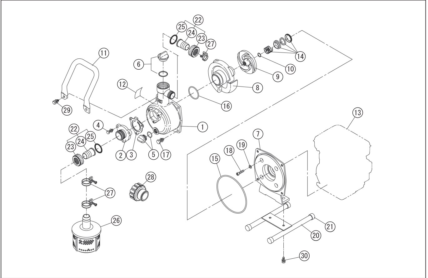
DWG No.012920801 MODELE : SEV-25F FORM : SEV-25F-BAC-0(K35)
