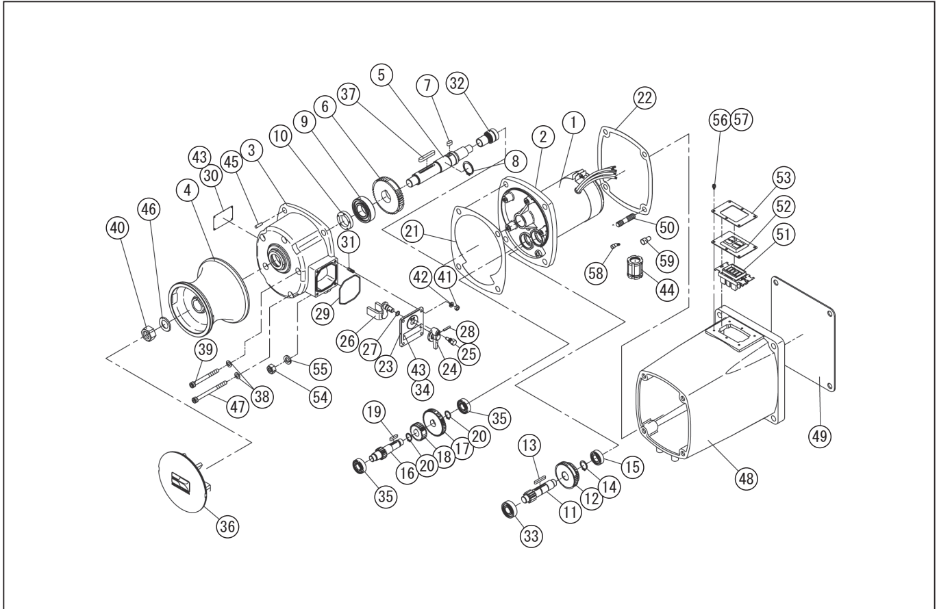
DWG No.027876105 MODELE : RES-4012 FORM : RES-4012-BAB-0 (400W·12V)
