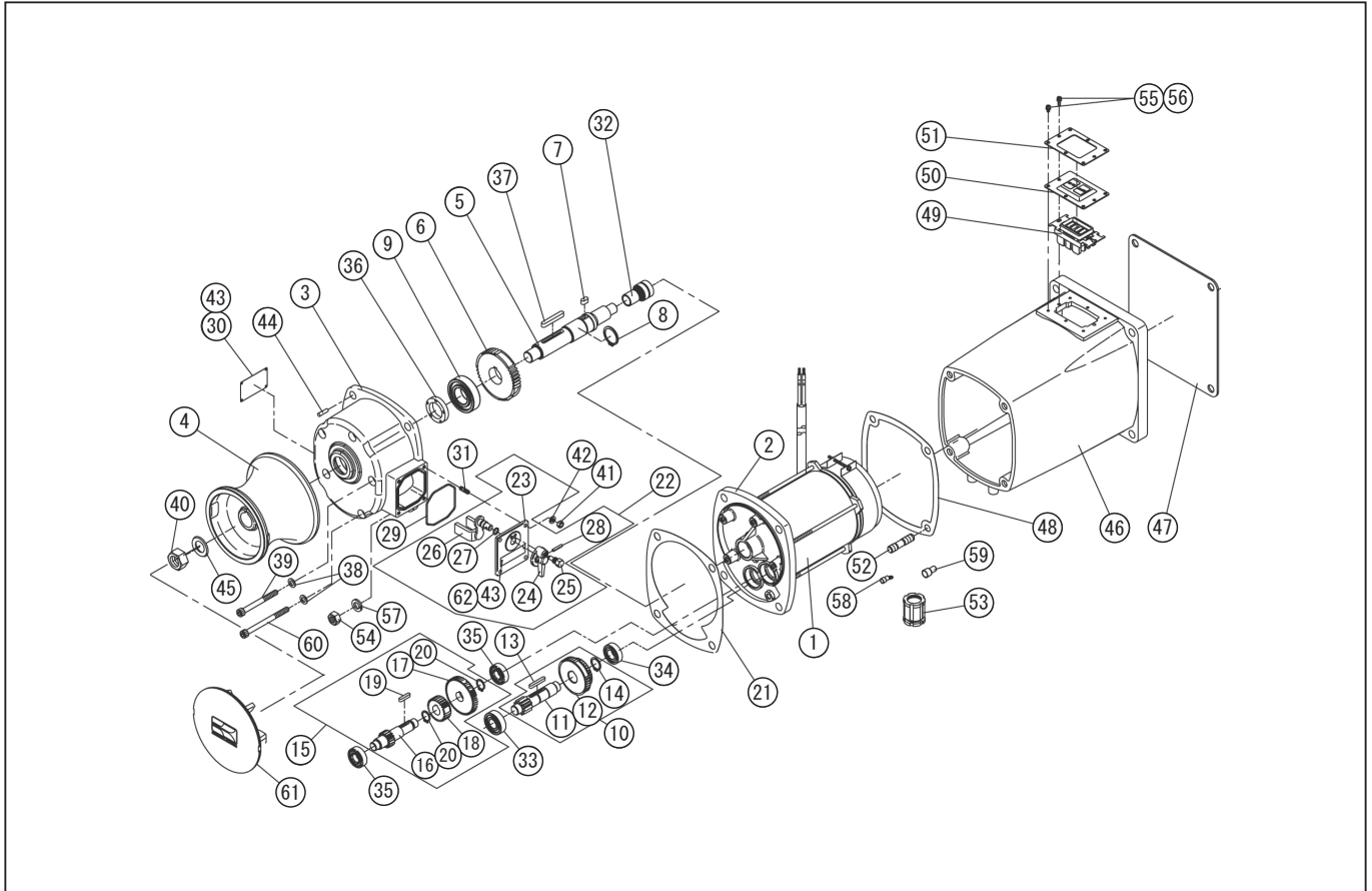
DWG No.027876003 MODELE : RES-4024 FORM : RES-4024-BAD-0
