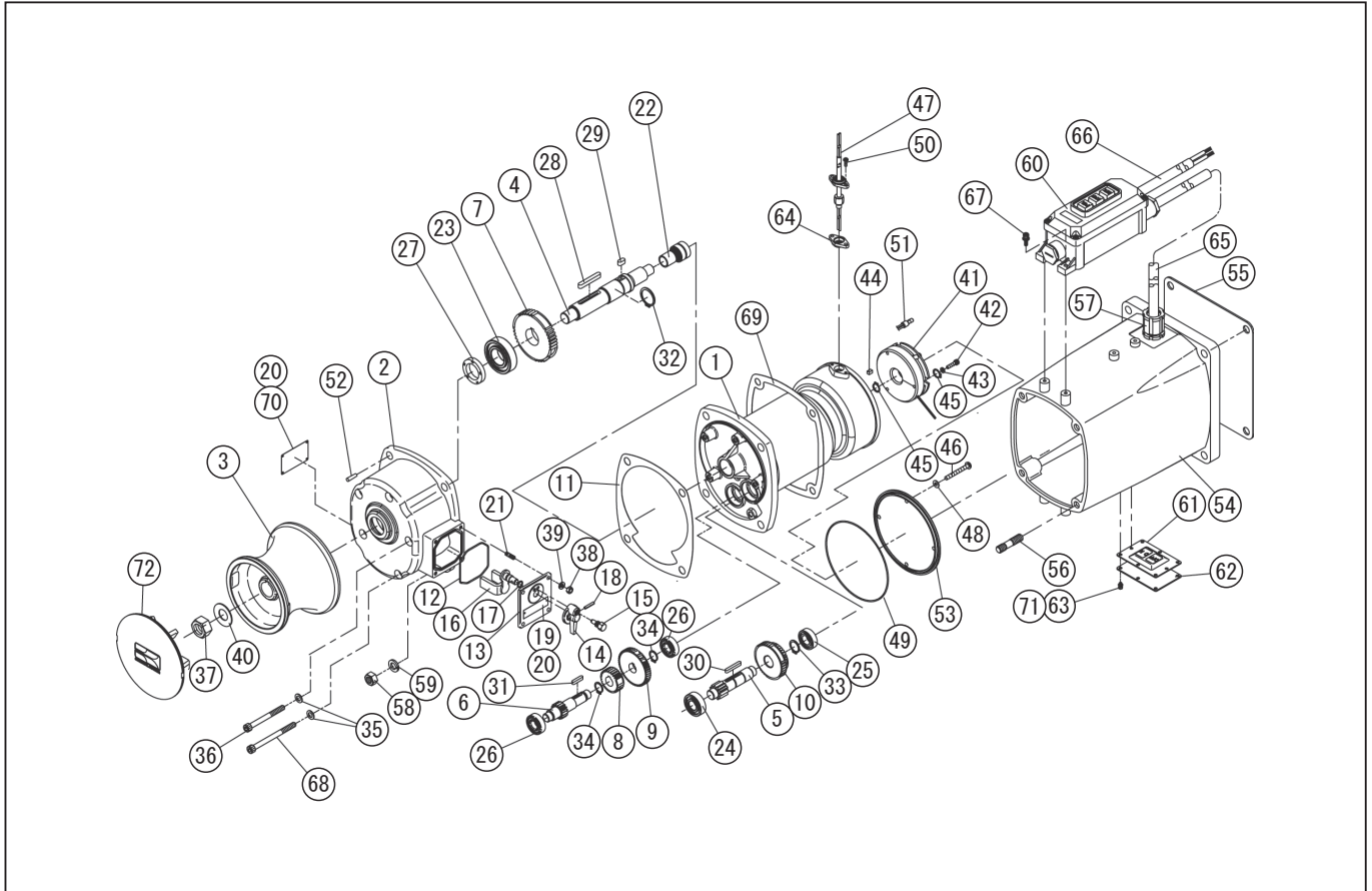
DWG No.027875602 MODELE : RES-5524LB FORM : RES-5524LB-BAD-0
