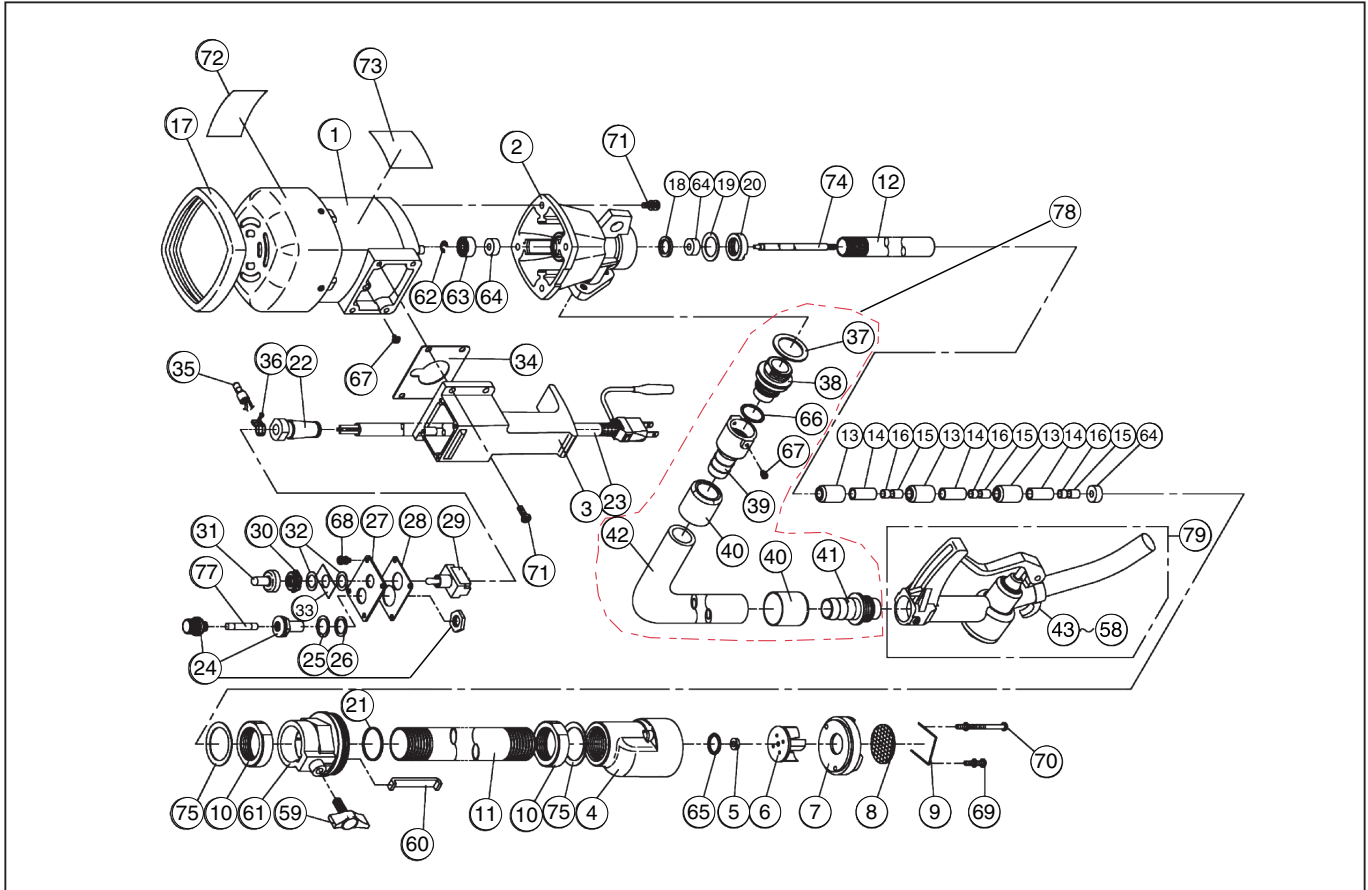
DWG No.004852617 MODEL:FA-100 FORM:FA-100-BAB-1
