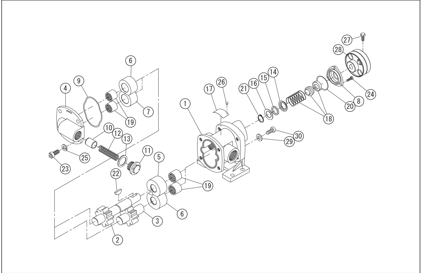
DWG No.007870806 MODEL : GL-40-10 FORM : GL-40-10-BAA-3
