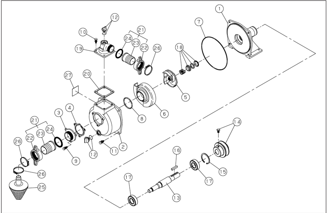
DWG No.066864904 MODEL : SU-50FC FORM : SU-50FC-BAA-1
